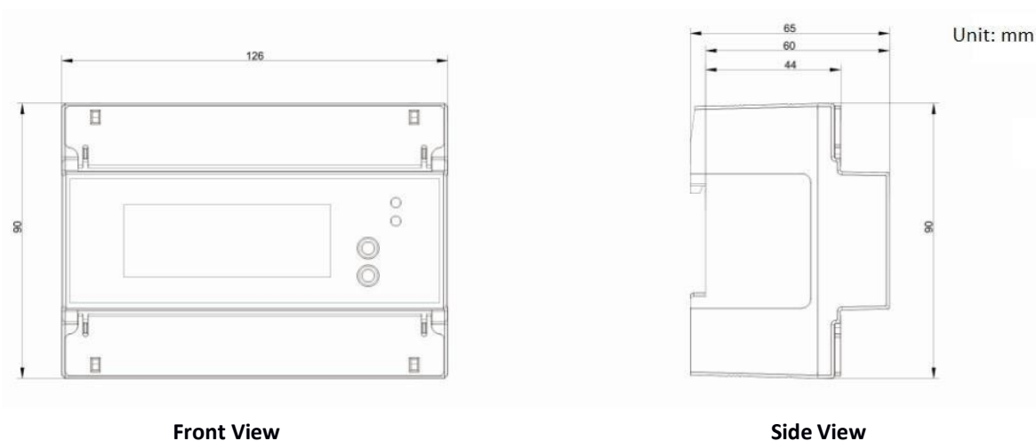
Figure 2-2 Dimensions
