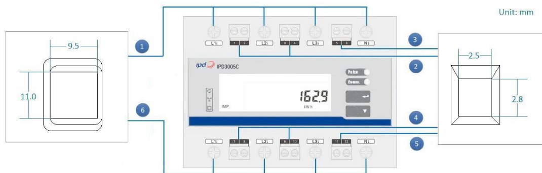
Figure 2-3 Terminal Dimensions
