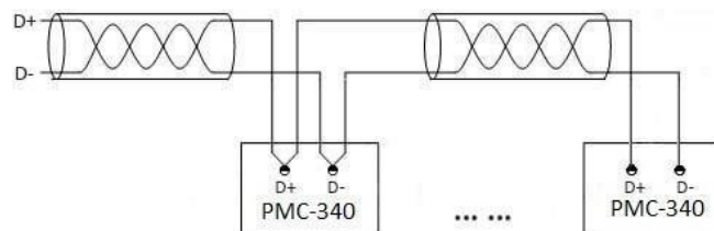
Figure 2-7 RS-485 Connections
