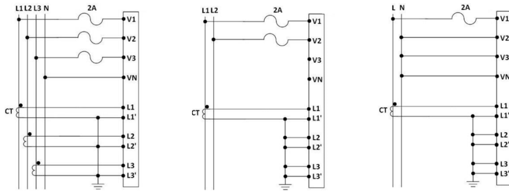
3P4W with 3CTs
